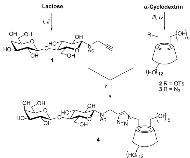
Scheme 2 i ) Neat propargylamine; ii ) Ac 2 O, MeOH (91% over 2 steps); iii ) TsCl, pyridine (26%); iv ) NaN 3 , DMF, 140 °C (93%); v ) CuSO 4 /sodium ascorbate, H 2 O/ i PrOH (75%).
